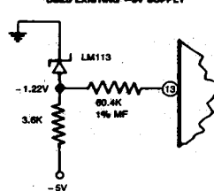
1.22V BAND GAP REFERENCE USES EXISTING -5V SUPPLY
