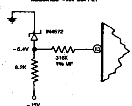
6.4V ZENER REFERENCE REQUIRES -15V SUPPLY
