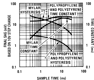
Dielectric Absorption Error in Hold Capacitor
