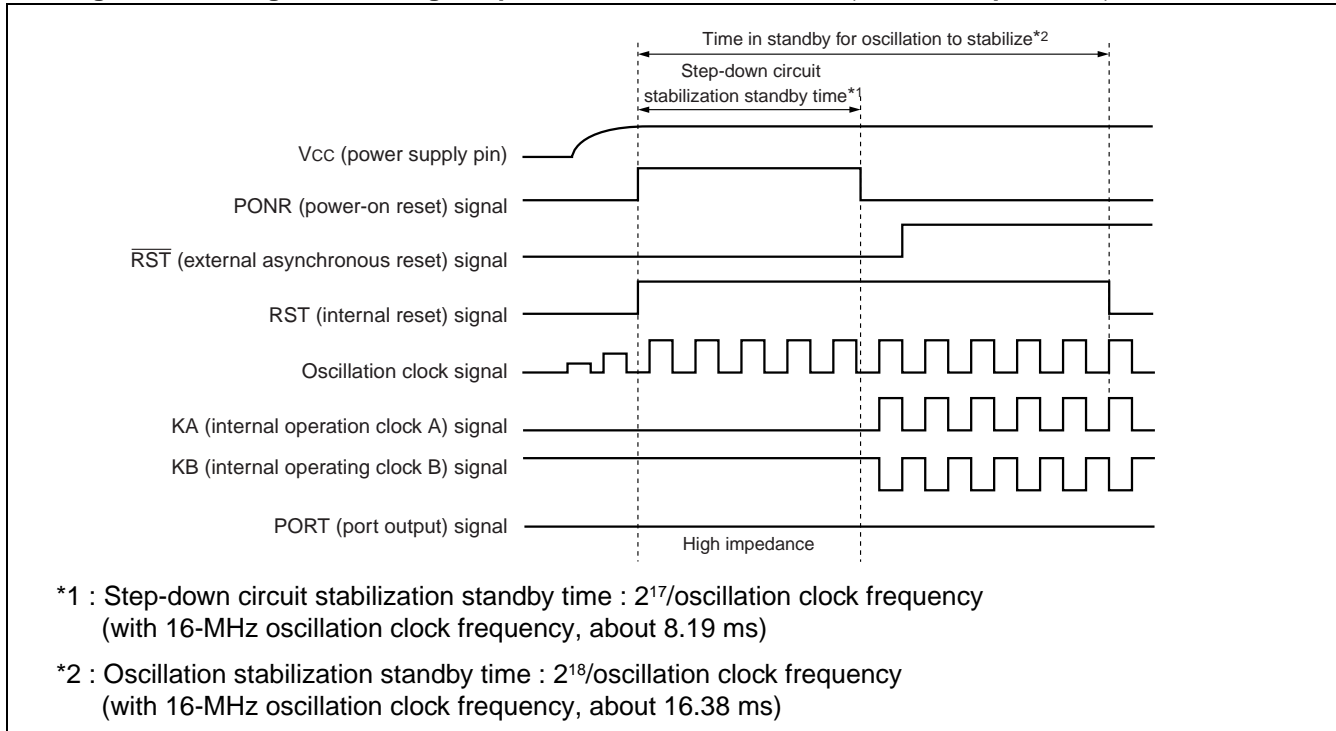
• Figure 2 - Timing Chart of High Impedance State for Ports 0/1 (when \overline{\text{RST}} pin is "L")
