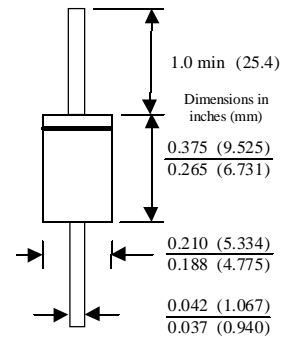
DO-201AE COLOR BAND DENOTES CATHODE
